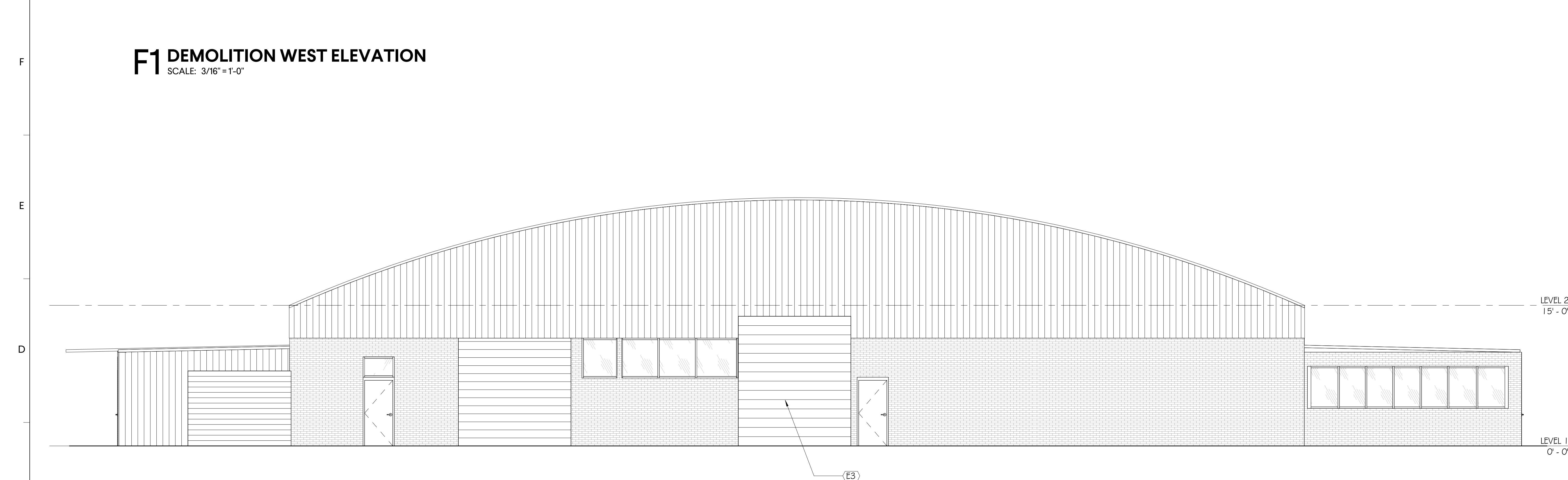
C1 NEW WORK WEST ELEVATION SCALE: 3/16" = 1'-0"
